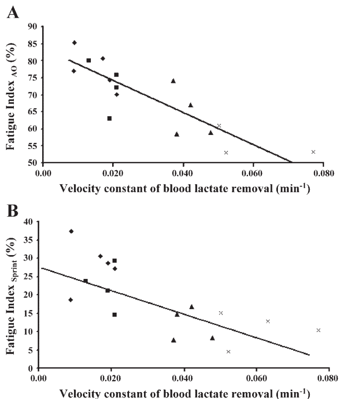
Fig. 5. Relationships between the fatigue index during the 1 min AO exercise test and the velocity constant of blood lactate removal \gamma_2 after the 1-min supramaximal AO test ( r = 0.85 , P < 0.001 , n = 16 ; A) and the fatigue index during the 10 short cycling sprints and the rate of blood lactate removal \gamma_2 ( r = 0.74 , P < 0.001 , n = 17 ; B). Symbols are as defined in Fig. 1.
