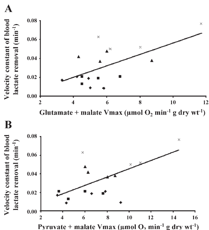
Fig. 2. Relationships between the velocity constant of blood lactate removal \gamma_2 after the 1-min supramaximal AO test and the glutamate + malate maximal ADP-stimulated respiration ( V_{\text{max}} ) ( r = 0.66 , P < 0.01 , n = 17 ; A) and the pyruvate + malate V_{\text{max}} ( r = 0.60 , P < 0.05 , n = 16 ; B). Glutamate + malate V_{\text{max}} and pyruvate + malate V_{\text{max}} (expressed in \mu\text{mol O}_2 \cdot \text{min}^{-1} \cdot \text{g dry wt}^{-1} ) are the V_{\text{max}} of the muscular fibers with glutamate + malate and pyruvate + malate as substrates. Symbols are as defined in Fig. 1 legend.
