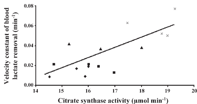
Fig. 1. Relationship between the velocity constant of blood lactate removal \gamma_2 after the 1-min supramaximal all-out (AO) test and the citrate synthase activity ( r = 0.76 , P < 0.01 , n = 15 ). \blacklozenge , Untrained subjects; \blacksquare , recreational athletes; \blacktriangle , middle-distance runners; \times , long-distance runners.
