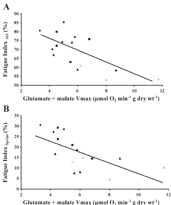
Fig. 3. Relationships between the fatigue index during the 1-min supramaximal AO exercise test and the glutamate + malate V_{\text{max}} ( r = 0.70 , P < 0.01 , n = 16 ; A) and the fatigue index during the 10 short cycling sprints and the glutamate + malate V_{\text{max}} ( r = 0.64 , P < 0.01 , n = 16 ; B). Symbols are as defined in Fig. 1 legend.
