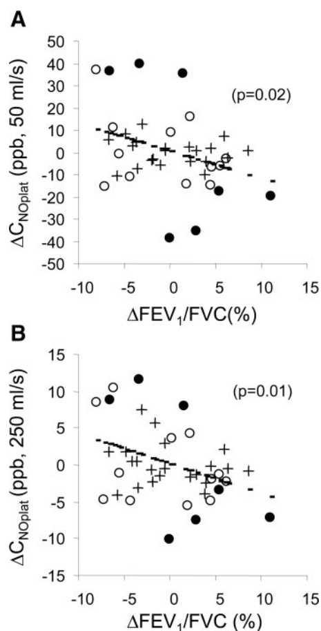
Fig. 8. Second-order partial correlation analysis demonstrates a significant inverse relationship between C_{NO,plat} and ratio of FEV_1 to FVC ( FEV_1/FVC ; % predicted) at an exhalation flow rate of 50 ml/s (A) and 250 ml/s (B) in a total of 44 subjects. +, HA ( n = 24 ); ○, ST ( n = 12 ); ●, SN ( n = 8 ).
