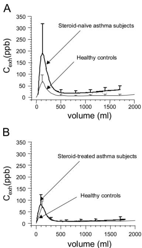
Fig. 4. A: composite experimental NO exhalation profiles are presented for the 20-s breath hold followed by a decreasing flow rate maneuver for steroid-naive (SN) asthma subjects (thick line) and healthy adults (HA) (thin line). B: composite experimental NO exhalation profiles are presented for the 20-s breath hold followed by a decreasing flow rate maneuver for steroid-treated (ST) asthma subjects (thick line) and HA (thin line). Values are means \pm SD.
